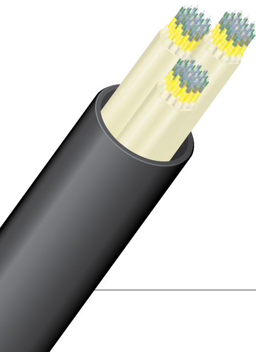
FIGURE 2: 4-in main conduit filled with bundled microducts providing 57 pathways, each filled with a 72-strand microcable.
